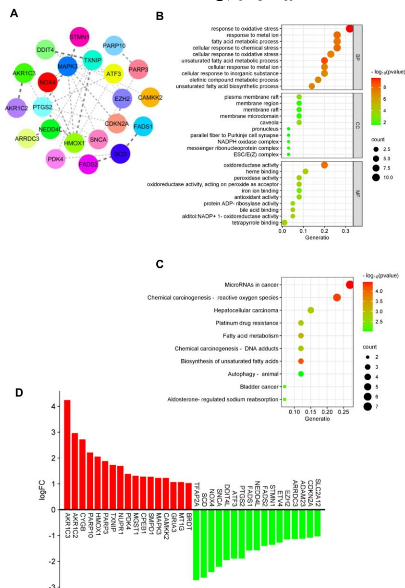
Figure 3. Analysis of FRDEGs. (A) PPI corresponding to FRDEGs. (B–C) GO and KEGG enrichment analysis of FRDEGs. (BP) biological process, (CC) cellular component and (MF) molecular function. (D) Comparison of differential expression of FRDEGs using logFC.
