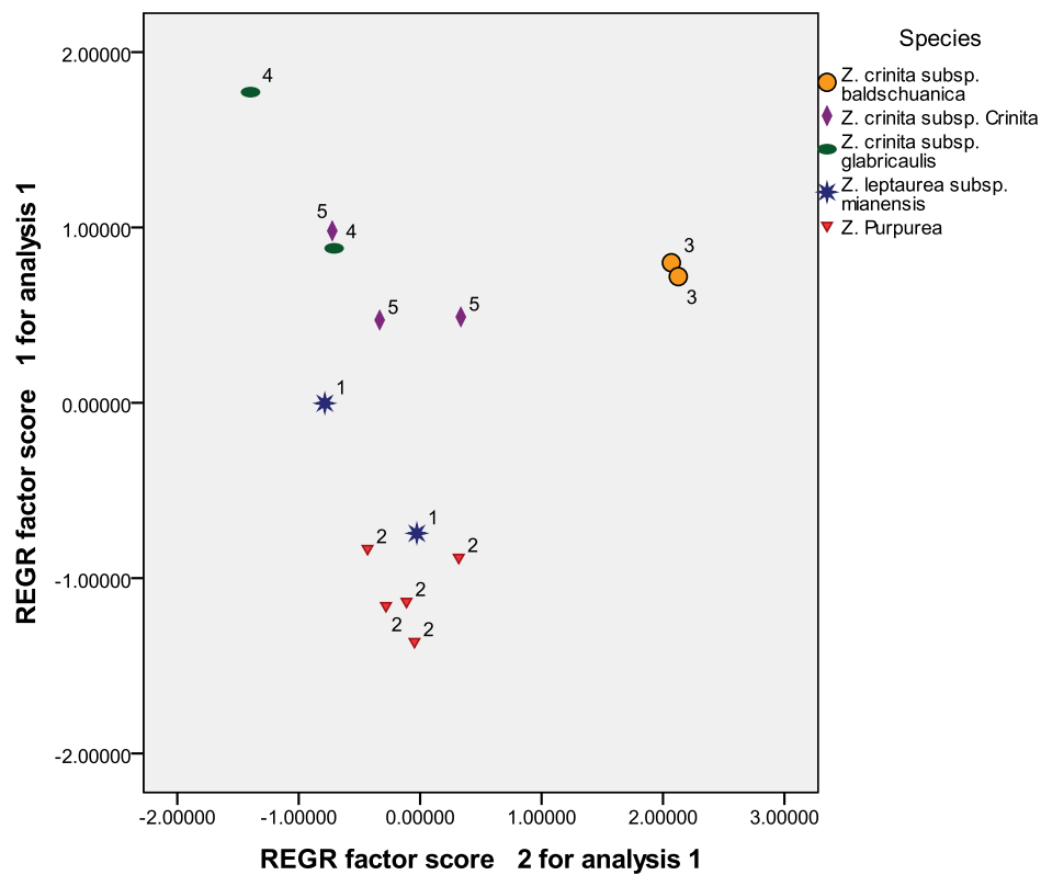
Fig. 9. PCA of the first and second factors based on Morphological quantitative cypsela features.
