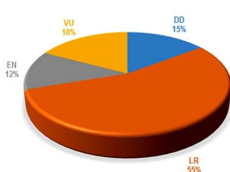
Fig. 8. A: The protected status of the families studied; B: the percentage of protected status; C: the protected status of endemic plants. DD: Data Deficiency, LR: Low Risk, EN: Endangered, VU: Vulnerable.
