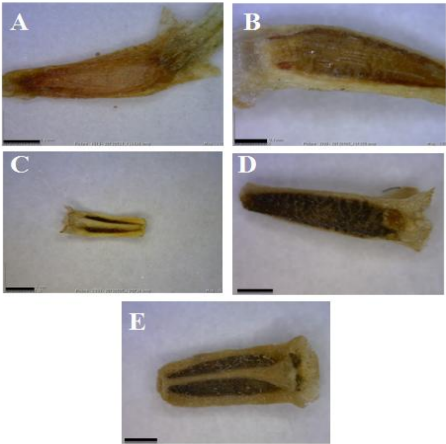
Fig. 3. Achene and pappus characters in Tripleurospermum species. A: T. caucasicum , B & C: T. monticolum , D & E: T. transcaucasicum ( A, B, D, E: scale bar=300 \mu m; C: scale bar= 600 \mu m).
