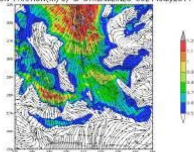
EMISSION FRICTION(m/s) & STREAMLINES 06Z14July2011
