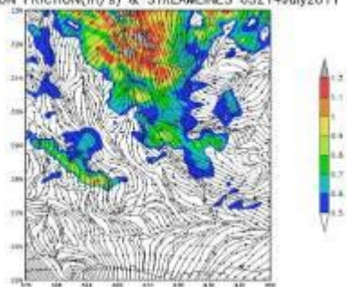
EMISSION FRICTION(m/s) & STREAMLINES 03Z14July2011
