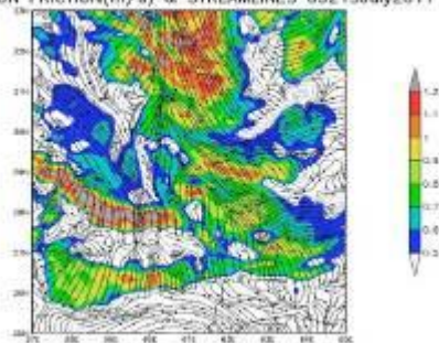
EMISSION FRICTION(m/s) &amp; STREAMLINES 03Z15July2011
