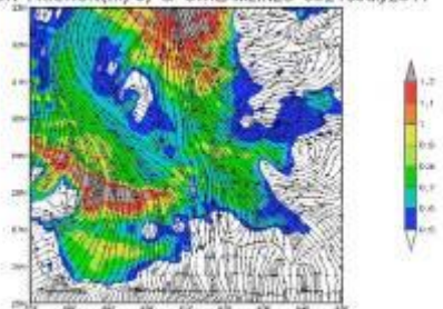
EMISSION FRICTION(m/s) &amp; STREAMLINES 09Z15July2011
