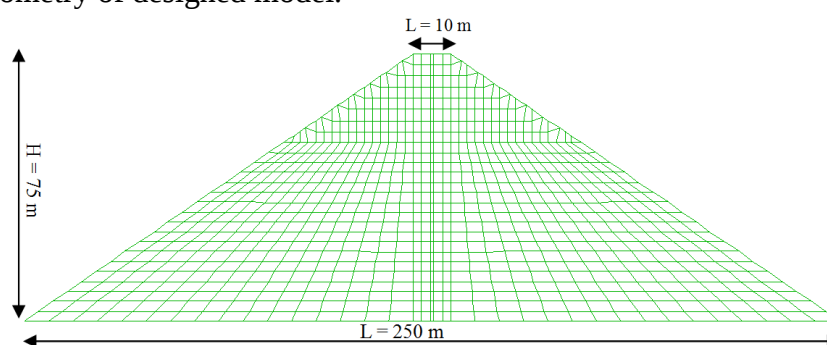
Fig. 2. Model of asphaltic core Rockfill dam, used in analyses
