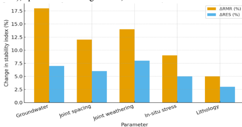
Fig. 13. Sensitivity of RMR and RES stability indices to \pm 10 – 30 % variation in dominant parameters.
