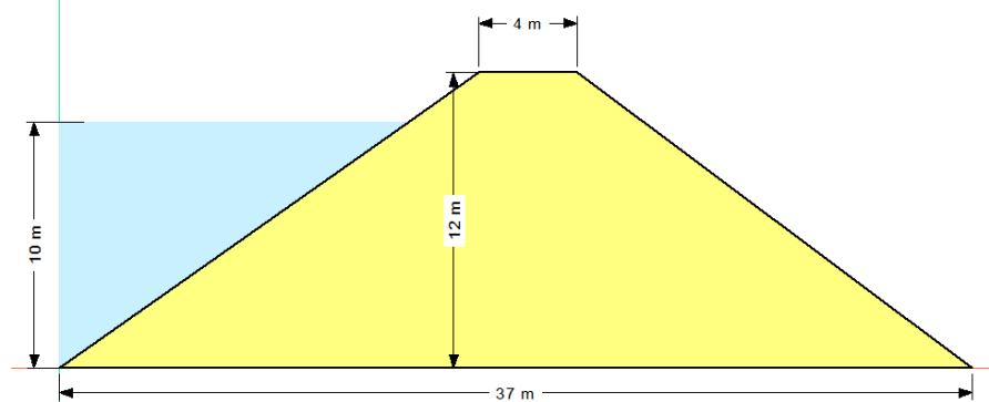
Fig. 3. Specifications of the Earth Dam
