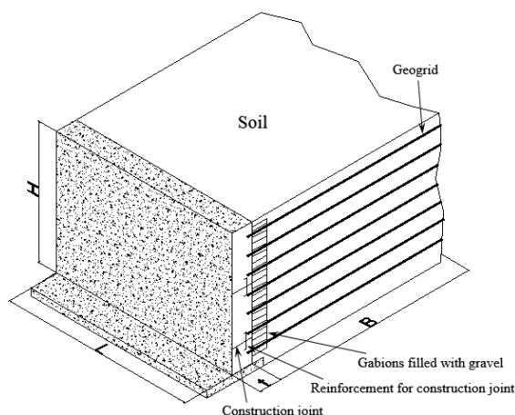
Figure 1. Schematic view of GRS-FHR wall
