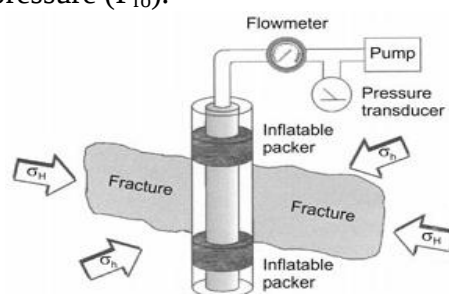
Figure1. Stages of starting hydraulic fracture test and the position of principle stresses to fracture plane [29]
